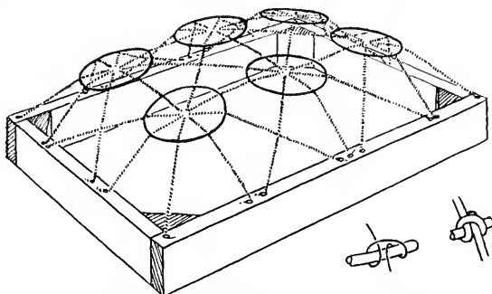
FIG. 484. SPRINGS TIED DOWN.
